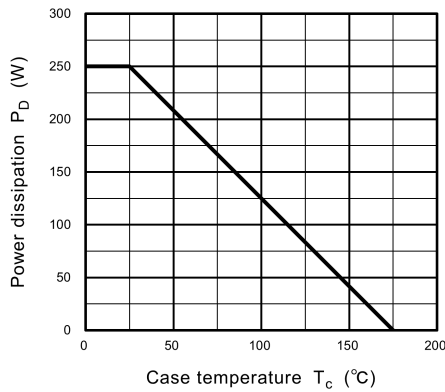
Fig. 8.14 P_D - T_c (Guaranteed Maximum)
