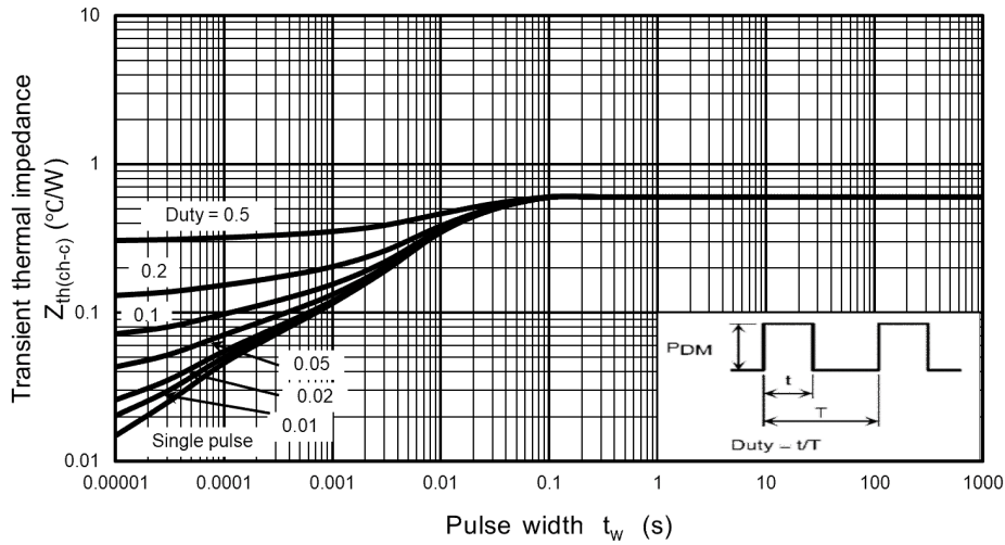
Fig. 8.13 Z_{th(ch-c)} - t_w (Guaranteed Maximum)
