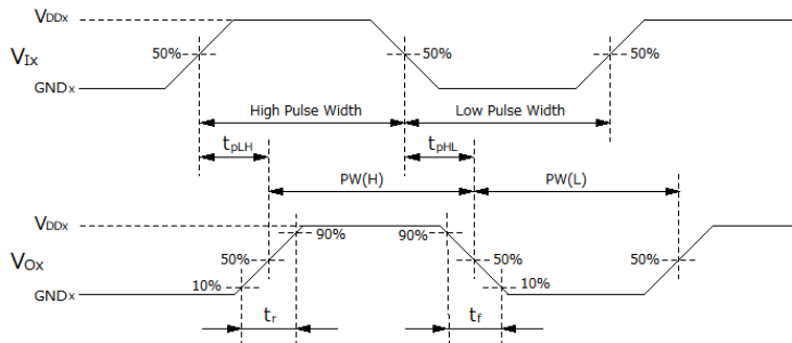
Fig. 12-2: DCL341x0B Switching Waveforms
