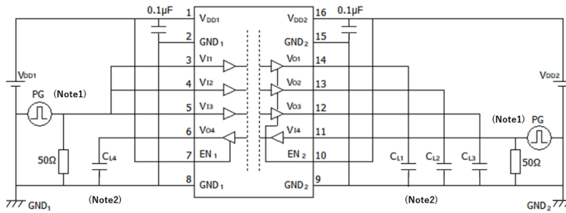
Fig. 12-1: DCL341L0B/DCL341H0B Switching Test Circuit
