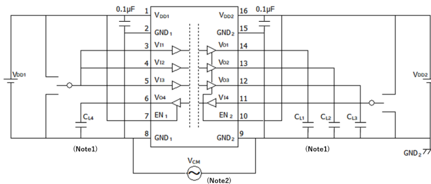
Fig. 12-5: DCL341L0B/DCL341H0B Common-Mode Transient Immunity Test Circuit
