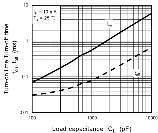
Fig. 11.9 t_{on}, t_{off} - C_L
