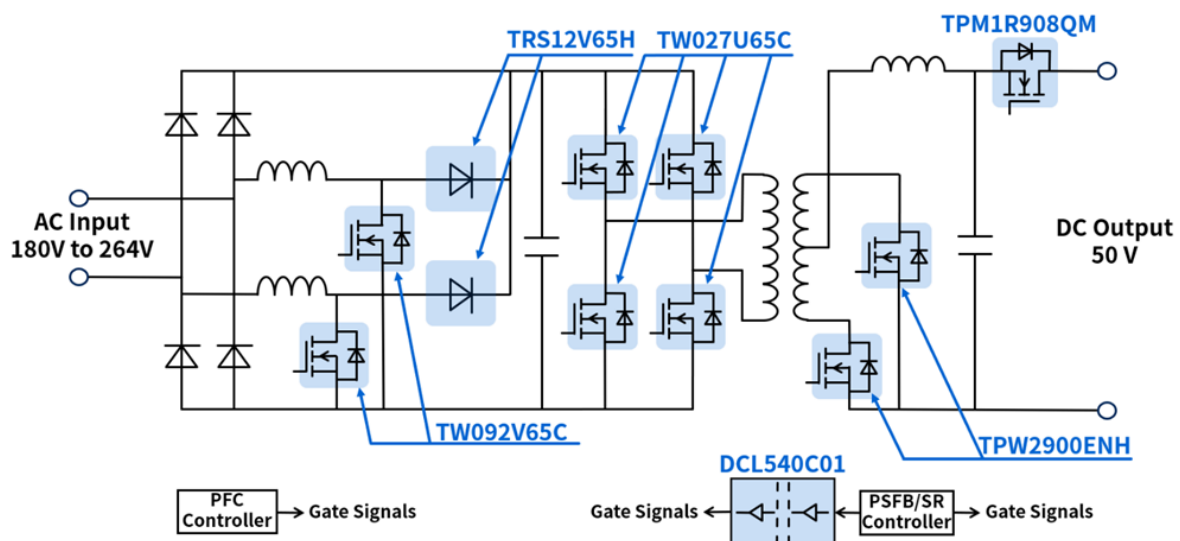
Fig. 2.1 Block Diagram
