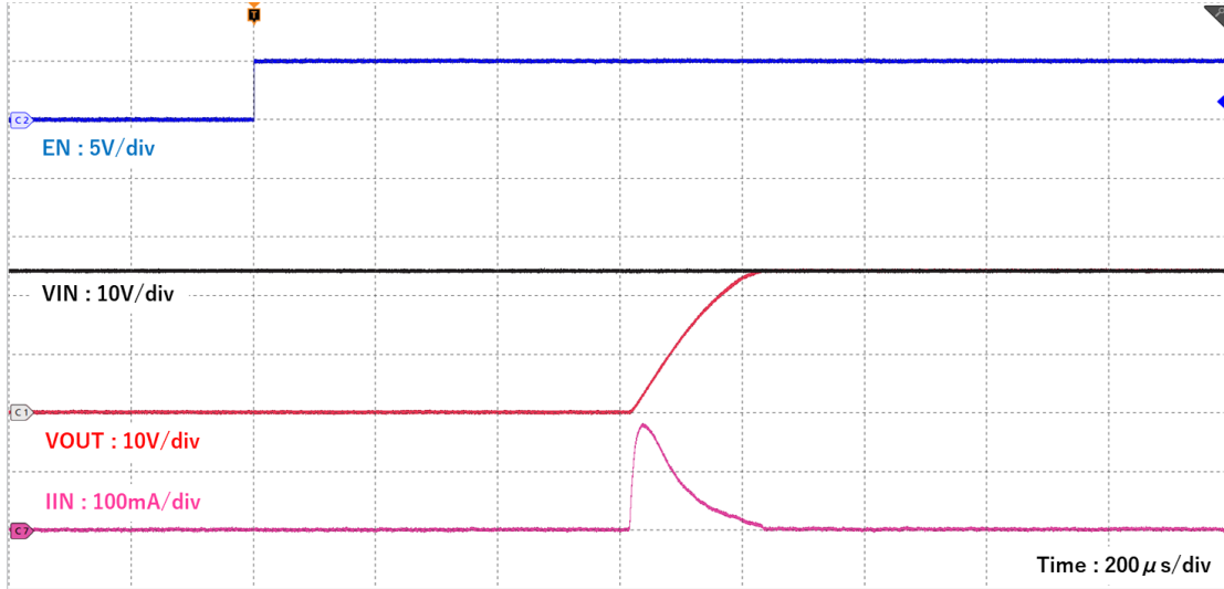
Figure 9.6.1 Waveform
