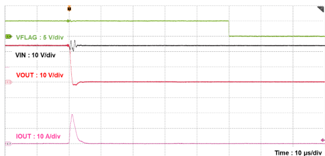
Figure 12.14 TCKE601RA Short-circuit protection (Zoom) V_{IN} = 24\text{ V} , C_{OUT} = 1\text{ }\mu\text{F} , R_{LIM} = 11\text{ k}\Omega , R_{OUT} = \text{Open to short}
