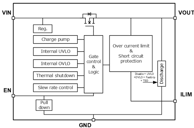
Figure 7.3 Block Diagram TCKE603RA,TCKE603RL
