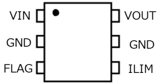
Figure 3.1 Pin Assignments TCKE601RA,TCKE601RL
