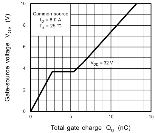
Fig. 7.8 Dynamic Input Characteristics
