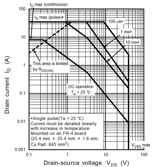
Fig. 7.10 Safe Operating Area
