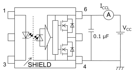
Fig. 13.1.5 I_{CCL} Test Circuit
