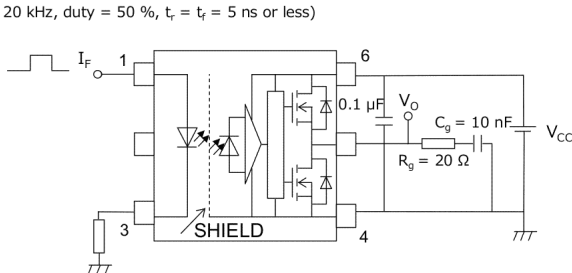
Fig. 13.1.6 Switching Time Test Circuit and Waveform
