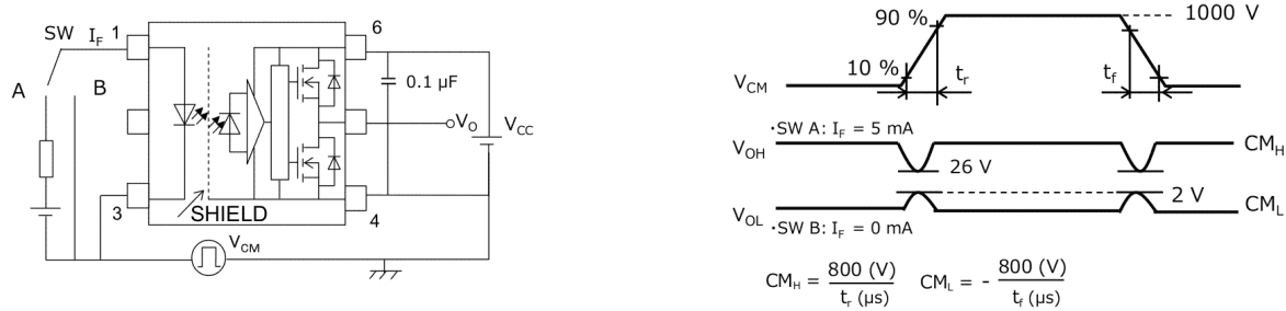
Fig. 13.1.7 Common-Mode Transient Immunity Test Circuit and Waveform
