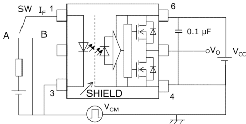
Fig. 13.1.7 Common-Mode Transient Immunity Test Circuit and Waveform
