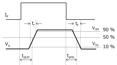
Fig. 13.1.6 Switching Time Test Circuit and Waveform
