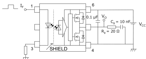
Fig. 13.1.6 Switching Time Test Circuit and Waveform
