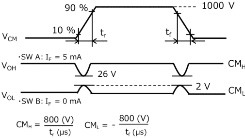
Fig. 13.1.7 Common-Mode Transient Immunity Test Circuit and Waveform
