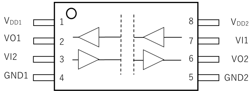
Figure 6.1 Pin Assignments (top view)
