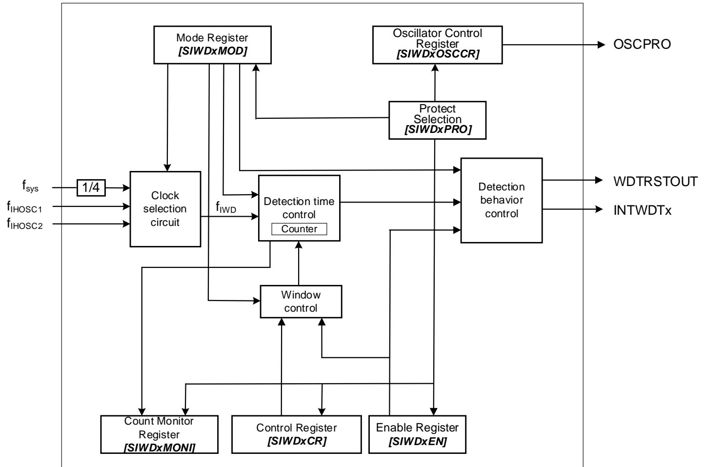
Figure 2.1 SIWDT Block Diagram
