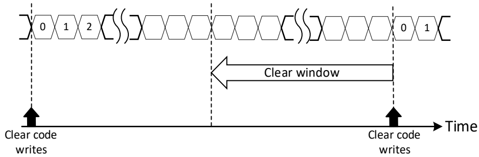
Figure 3.1 Clear Code Writes during Clear Window Interval
