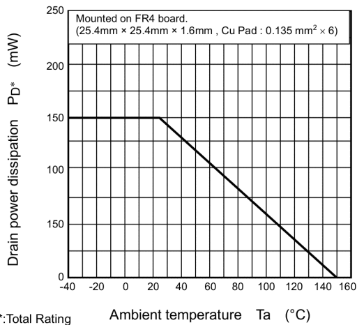
Fig. 7.11 P_{D^*} - T_a
