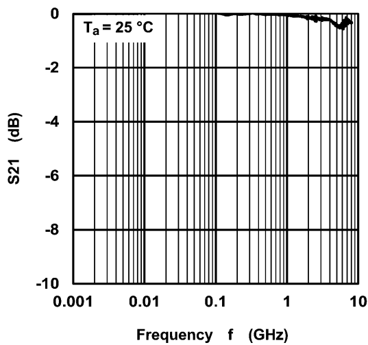
図 9.1 S_{21} - f
