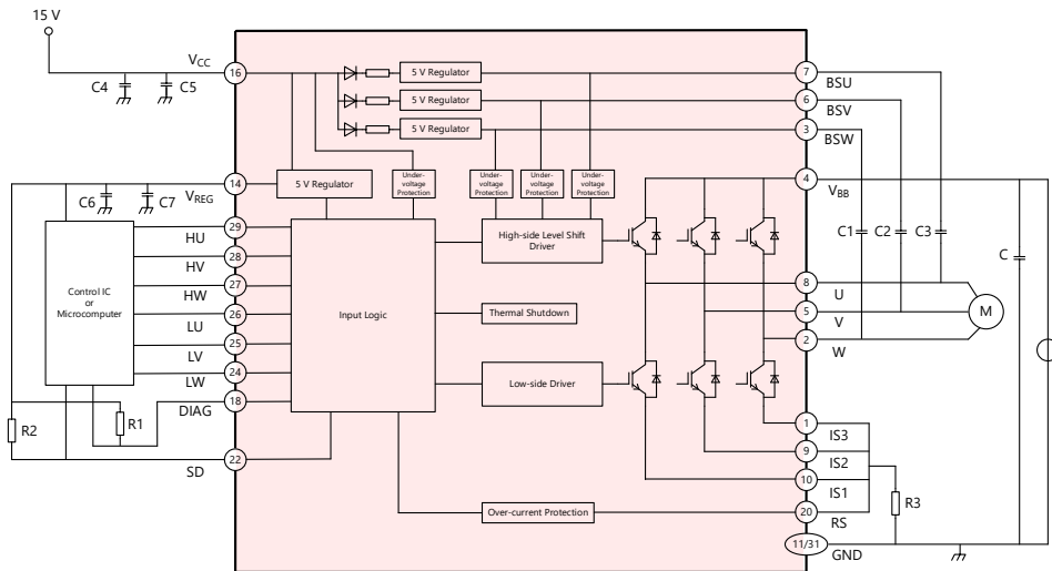
TPD4163F Application Circuit Example
