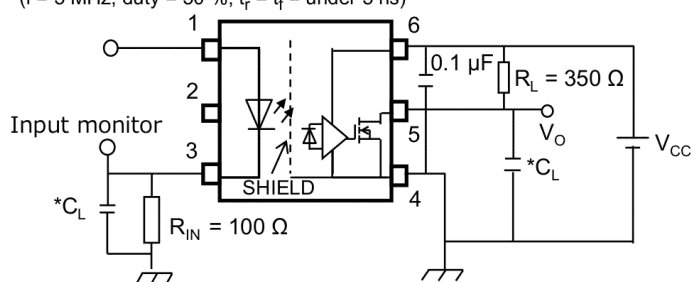
Fig. 13.1.6 Switching Time Test Circuit and Waveform
