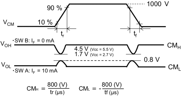
Fig. 13.1.7 Common-Mode Transient Immunity and Waveform
