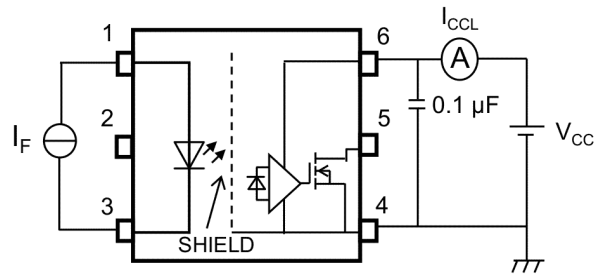
Fig. 13.1.4 ICCL Test Circuit
