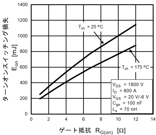
図 8.11 E_{on} - R_{G(off)}
