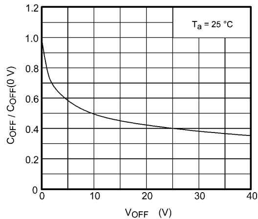
Fig. 12.11 C_{OFF}/C_{OFF}(0\text{V}) - V_{OFF}
