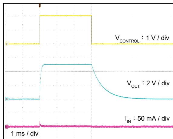
V_{OUT} = 5.0 \text{ V} ( V_{IN} = 24.0 \text{ V} )
