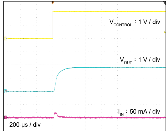
V_{OUT} = 1.8 V ( V_{IN} = 24.0 V )
