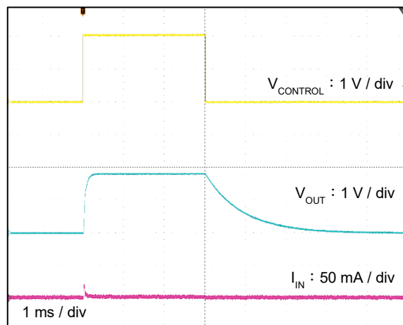
V_{OUT} = 1.8 \text{ V} ( V_{IN} = 24.0 \text{ V} )
