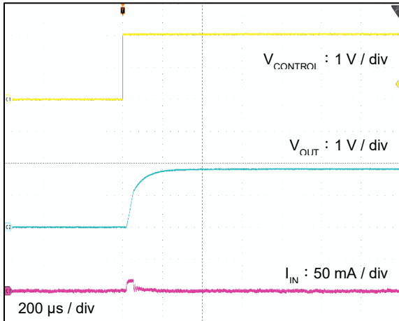
V_{OUT} = 1.8 V ( V_{IN} = 4.0 V )
