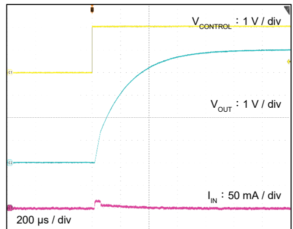
V_{OUT} = 5.0 V ( V_{IN} = 24.0 V )
