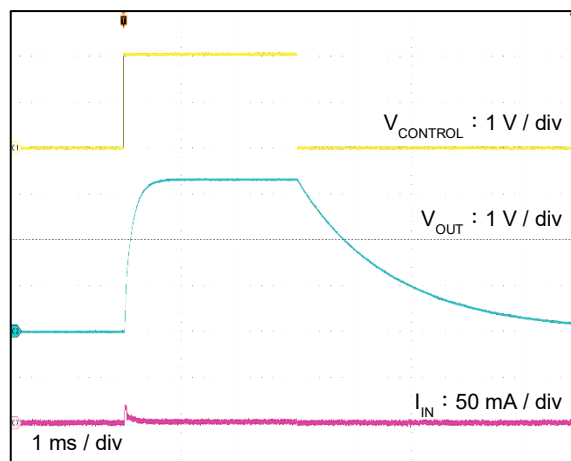
V_{OUT} = 3.3 \text{ V} ( V_{IN} = 24.0 \text{ V} )
