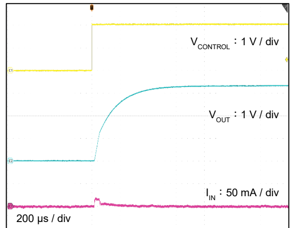
V_{OUT} = 3.3 V ( V_{IN} = 24.0 V )
