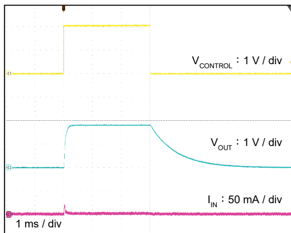
V_{OUT} = 1.8 \text{ V} ( V_{IN} = 4.0 \text{ V} )
