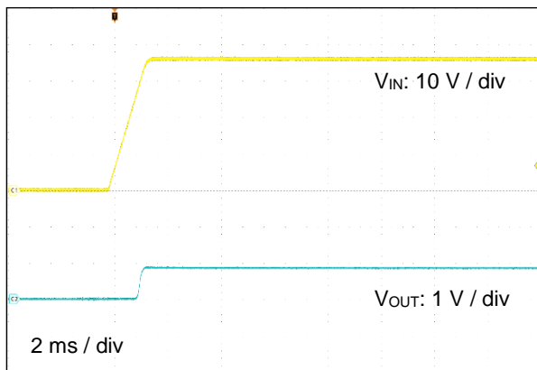
TCR1HF33B, V IN = 0 V to 36 V, No Load
