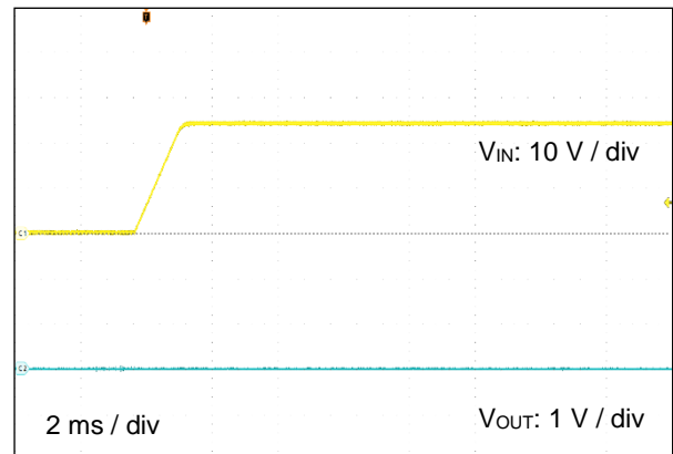
TCR1HF33B, V IN = 0 V to 24 V, No Load
