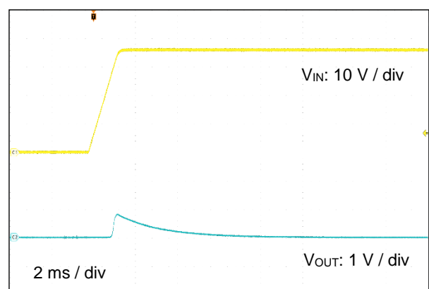
TCR1HF33B, V IN = 0 V to 36 V, No Load
