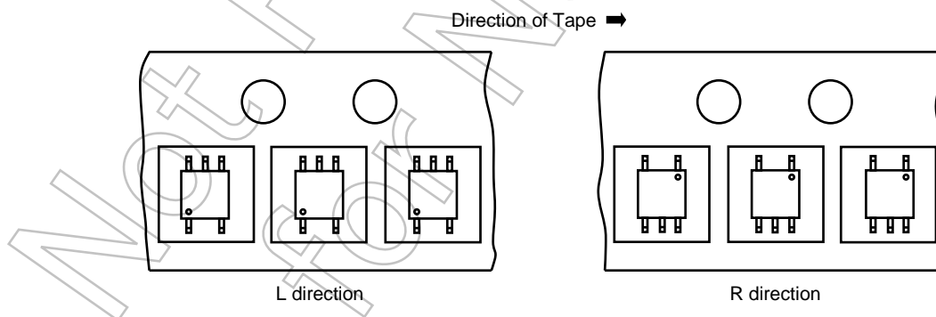
Figure 1 Device Orientation
