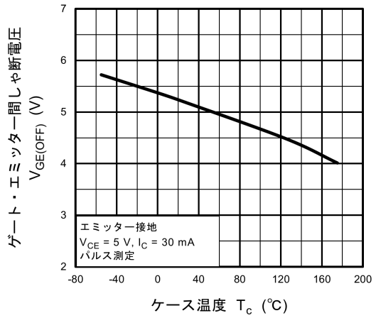
図 8.8 V_{GE(OFF)} - T_C
