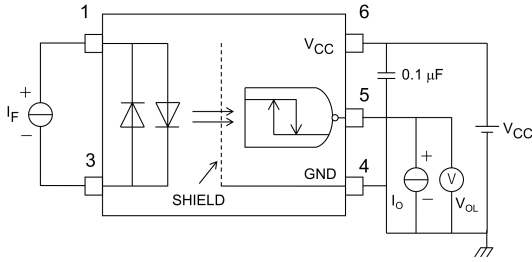
Fig. 12.1.1 V_{OL} Test Circuit
