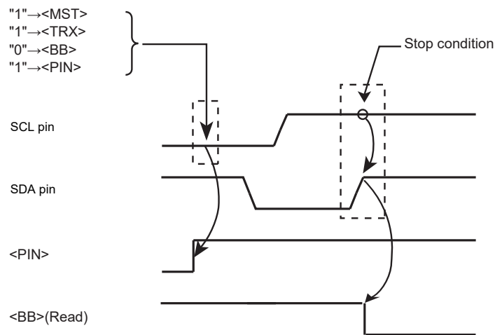
Figure 12-13 Generating the Stop Condition
