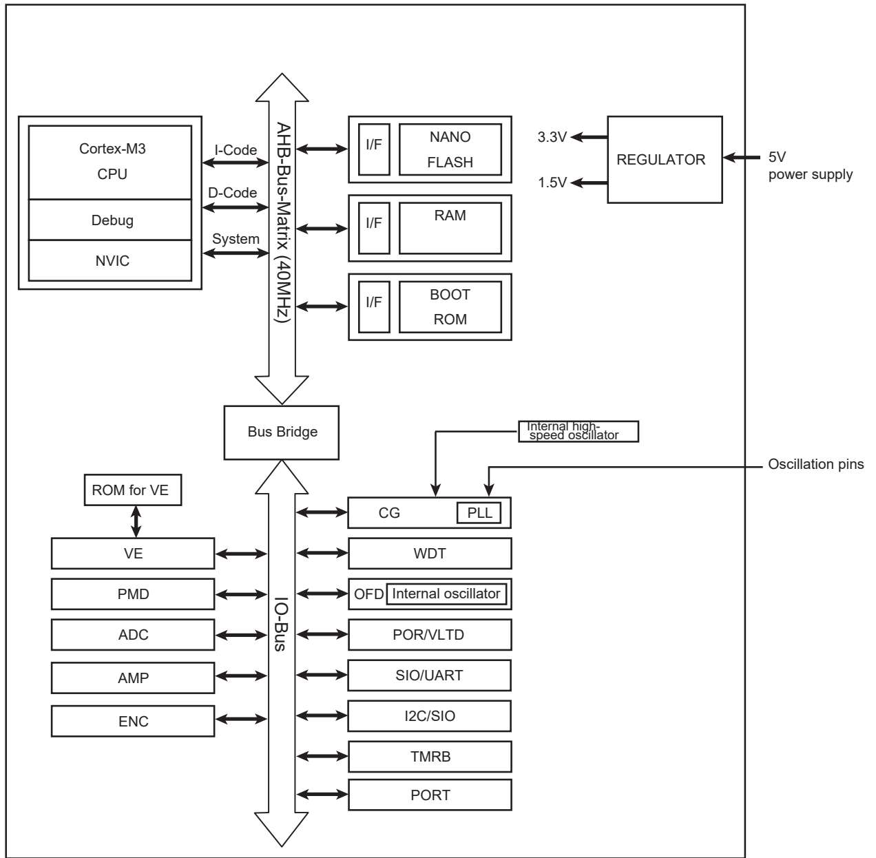
Figure 1-1 TMPM375FSDMG block diagram
