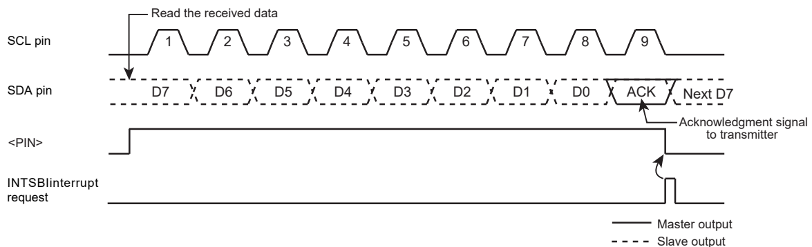
Figure 12-11 \langle BC[2:0] \rangle = "000" , \langle ACK \rangle = "1" (Receiver Mode)
