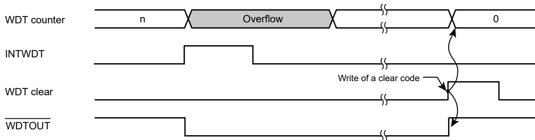
Figure 21-2 INTWDT interrupt generation
