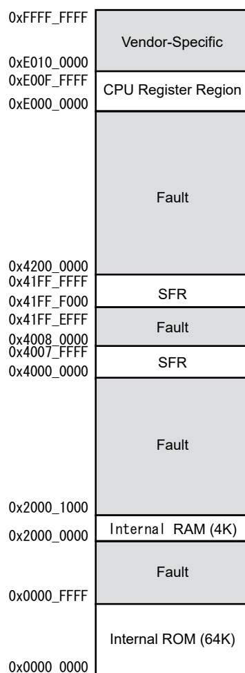
Figure 3-1 Memory Map
