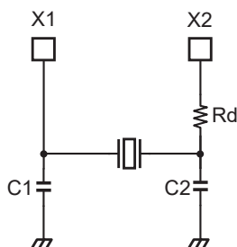
Figure 25-5 Example of high-frequency oscillation circuit
