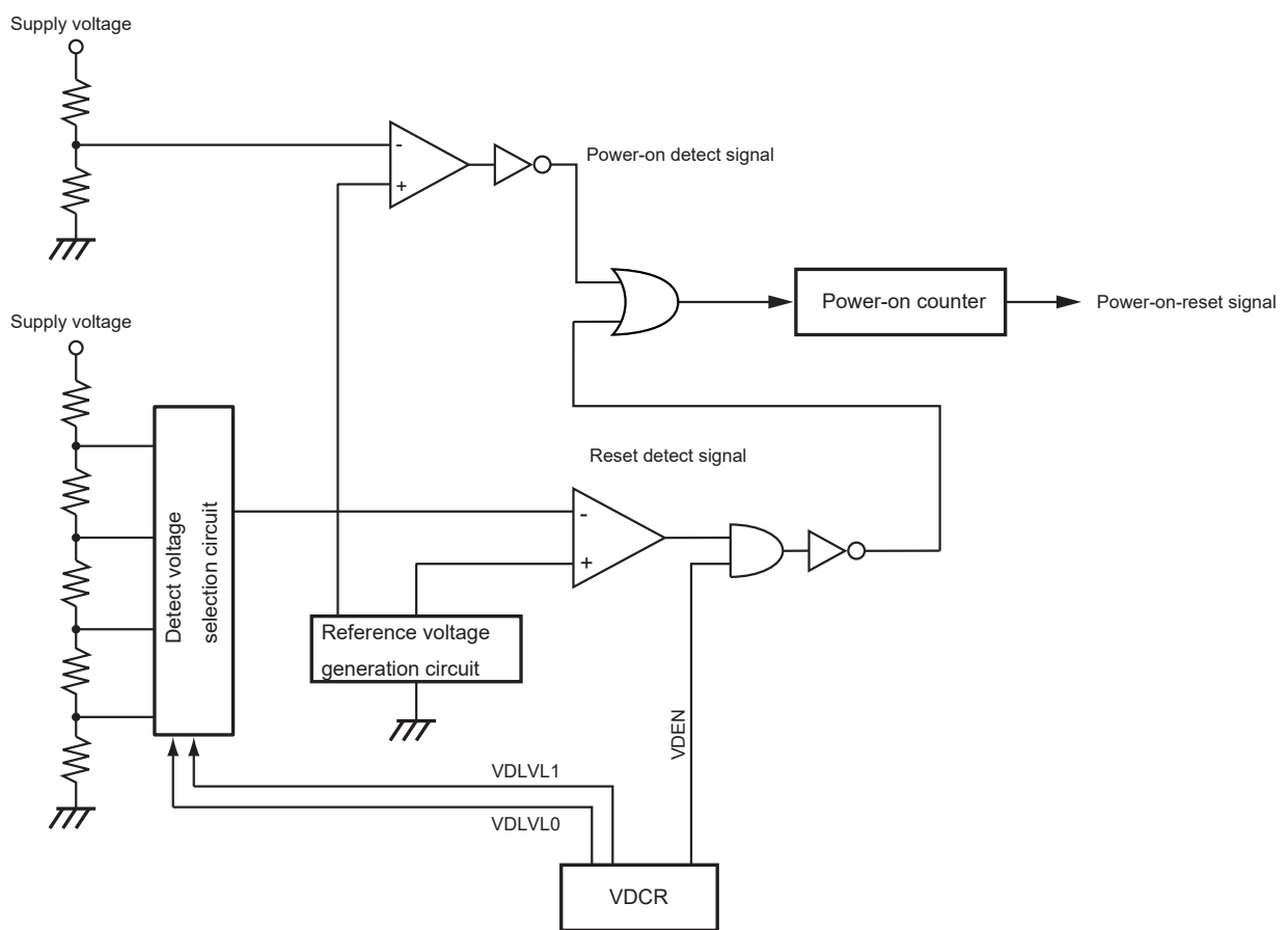
Figure 18-1 Power-on-reset circuit
