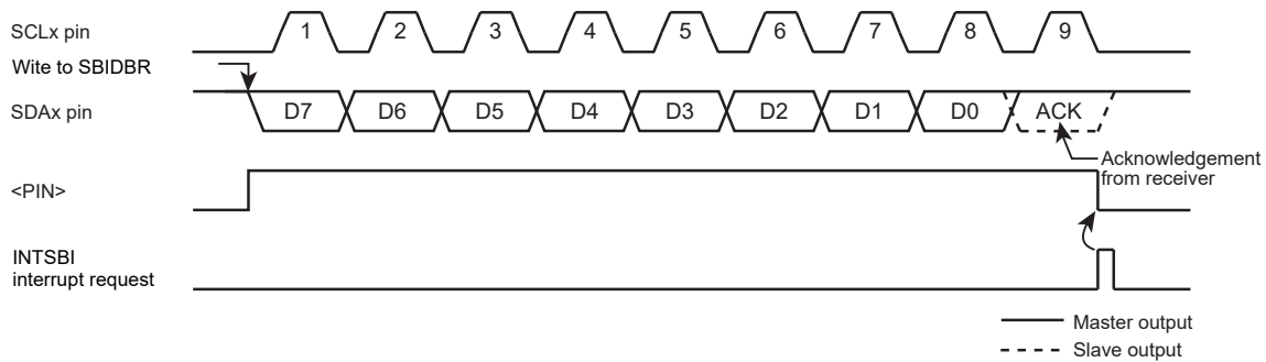
Figure 12-10 \langle BC[2:0] \rangle = "000" , \langle ACK \rangle = "1" (Transmitter Mode)
