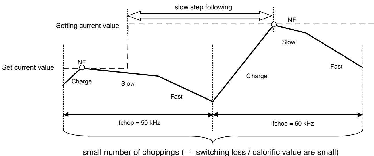
Figure 4.3 Constant current waveform (when f_{CHOP} = 50 kHz)
