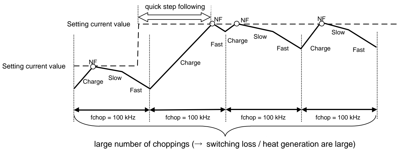
Figure 4.2 Constant current waveform (when f_{CHOP} = 100 kHz)
