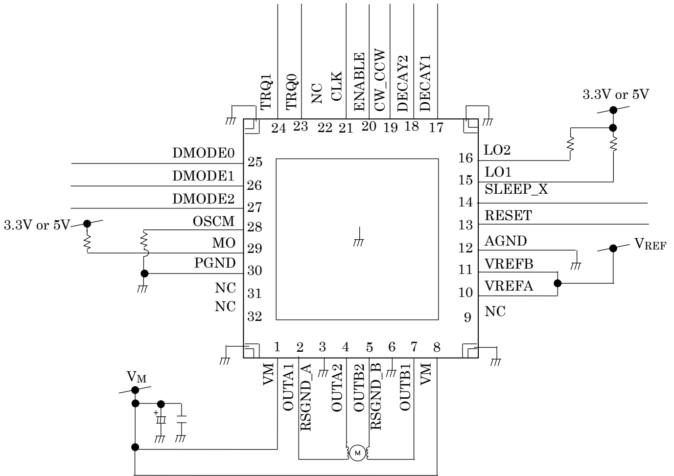
Figure 7.1 Application circuit example
