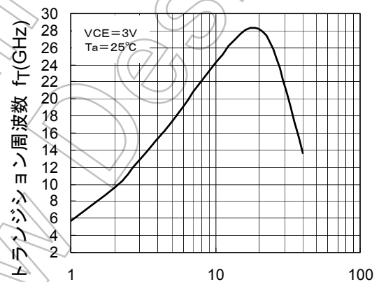
f_T-I_C
