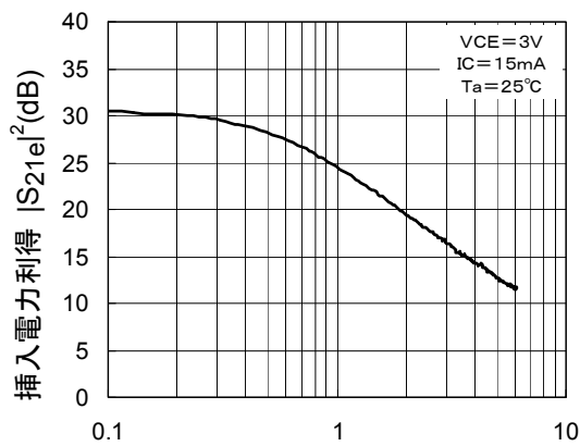
|S_{21e}|^2 -Freq.
