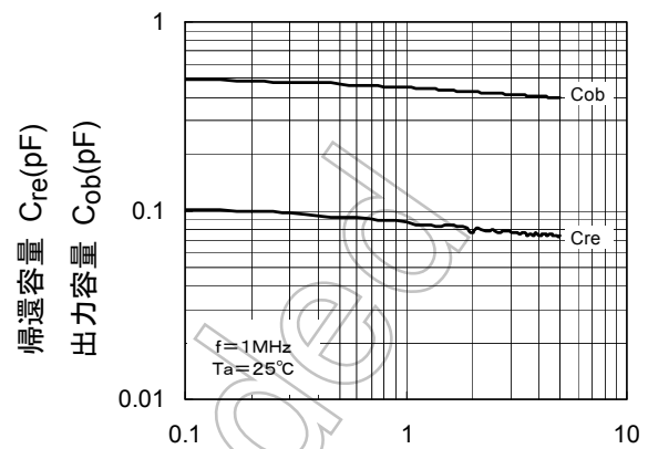
C_{re}, C_{ob} - V_{CB}
