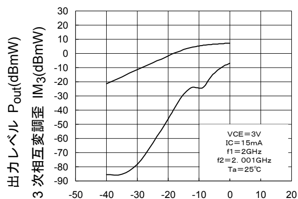
P_{out}, IM_3-P_{in}
