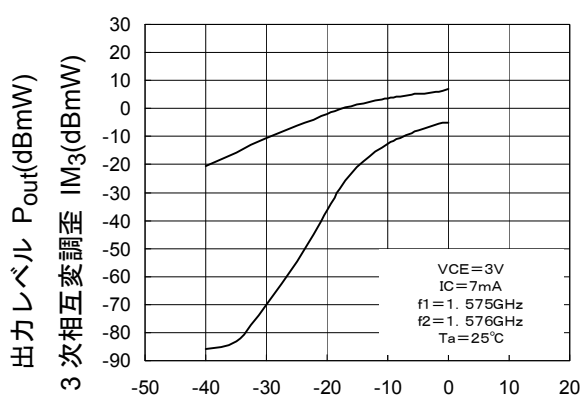
P_{out}, IM_3-P_{in}
