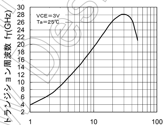
f_T-I_C
