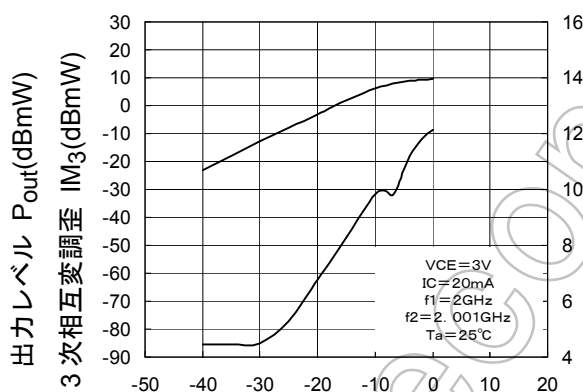
P_{out}, IM_3-P_{in}
