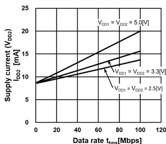
Fig.13.6. DCL542x01 I_{DD2} Supply Current - Data rate
