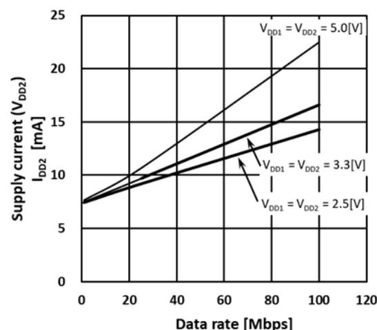
Fig.13.4. DCL541x01 I_{DD2} Supply Current - Data rate
