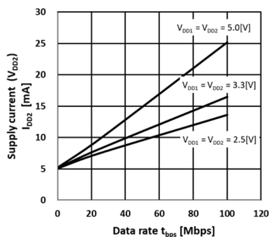
Fig.13.2. DCL540x01 I_{DD2} Supply Current - Data rate
