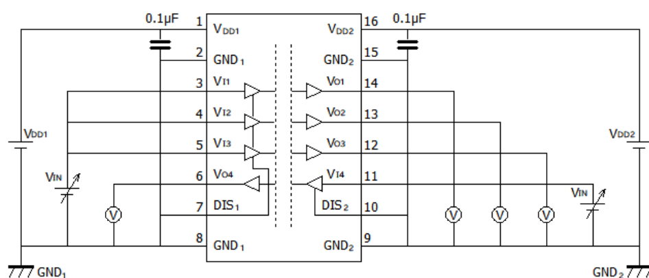
Fig.12.3.5. DCL541A01/DCL541B01 V_{IH}/V_{IL} Test Circuit
