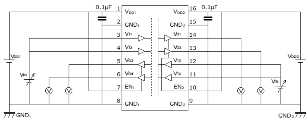
Fig.12.3.4. DCL542L01/DCL542H01 V_{IH}/V_{IL} Test Circuit
