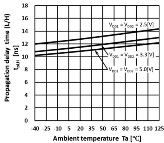
Fig.13.9. Propagation Delay Time t_{pLH} - T_a
