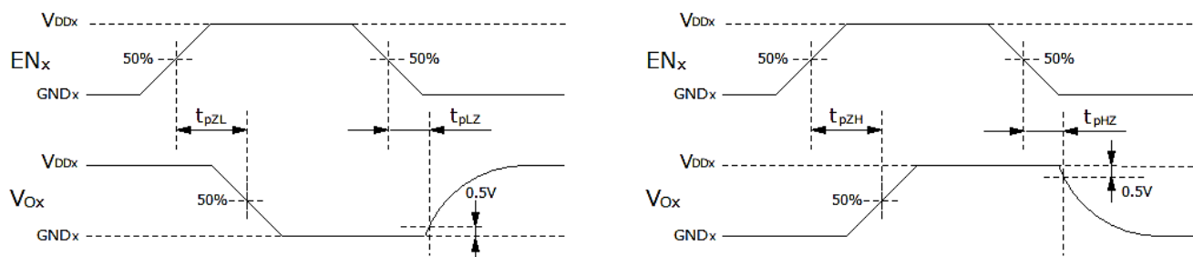
Fig.12.5.4. DCL54xL01/ DCL54xH01 Enable propagation delay time waveform
