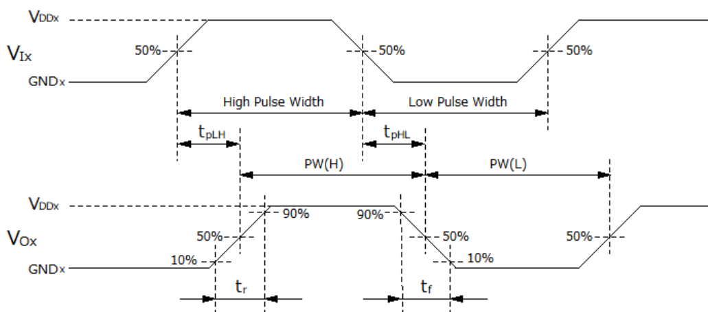
Fig.12.4.6. DCL54xx01 Switching characteristic waveform diagram
