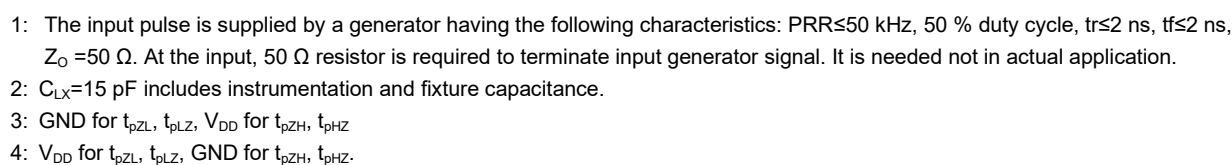
Fig.12.5.3. DCL541L02/ DCL542H01 Enable Propagation Delay Time Test Circuit
