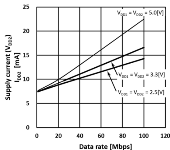
Fig.13.4. DCL5401x01 I_{DD2} Supply Current - Data rate
