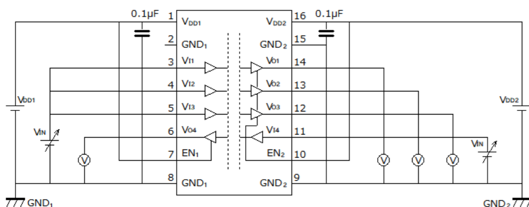
Fig.12.3.3. DCL541L01/DCL541H01 V_{IH}/V_{IL} Test Circuit
