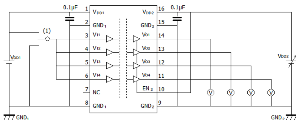
Fig.12.1.7. DCL540L01/DCL540H01 VDD2UV+/ VDD2UV-Test Circuit
