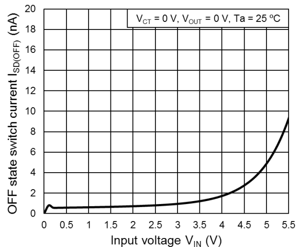
I_{SD(OFF)} - V_{IN}
