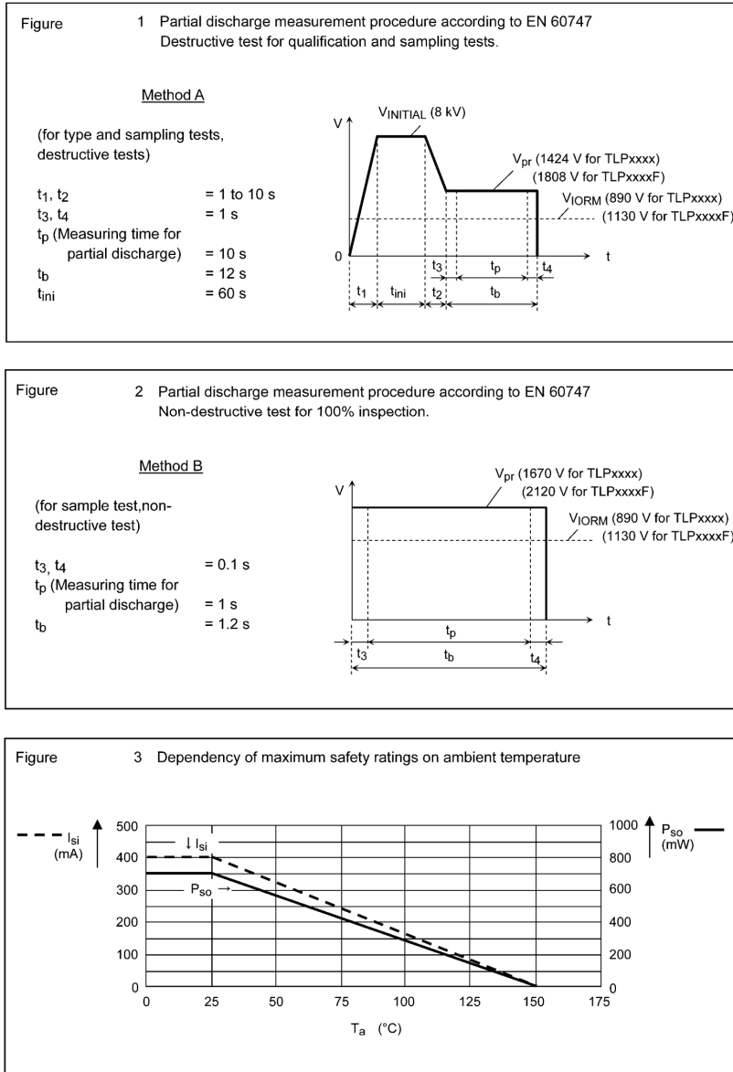
Fig. 17.3 Measurement Procedure
