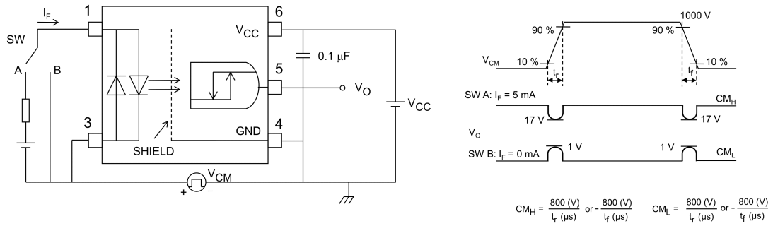
Fig. 12.1.9 Common-Mode Transient Immunity Test Circuit and Waveform
