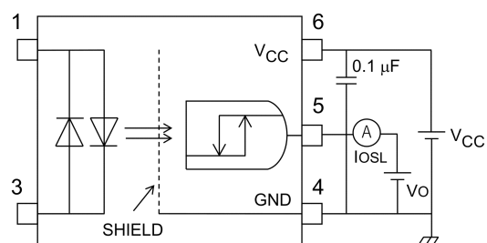
Fig. 12.1.5 I_{OSL} Test Circuit
