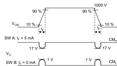
Fig. 12.1.8 Switching Time Test Circuit and Waveform
