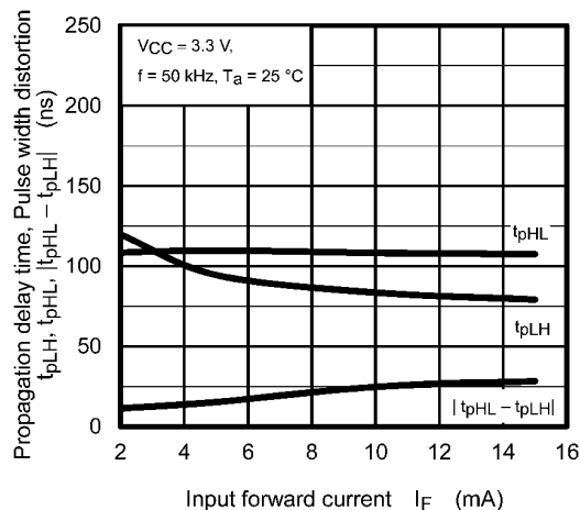
Fig. 12.2.22 t_{pHL} , t_{pLH} , |t_{pHL} - t_{pLH}| - I_F (Test Circuit Fig. 12.1.8)
