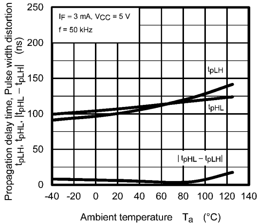
Fig. 12.2.19 t_{pHL} , t_{pLH} , |t_{pHL}-t_{pLH}| - T_a (Test Circuit Fig. 12.1.8)
