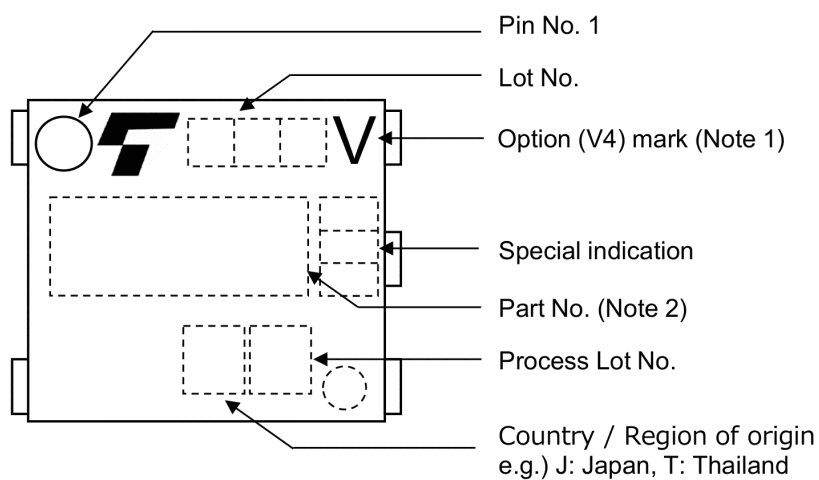
Fig. 16.4 Marking Example
