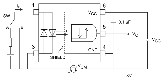
Fig. 12.1.9 Common-Mode Transient Immunity Test Circuit and Waveform
