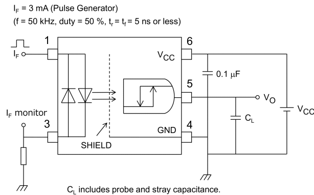
Fig. 12.1.8 Switching Time Test Circuit and Waveform
