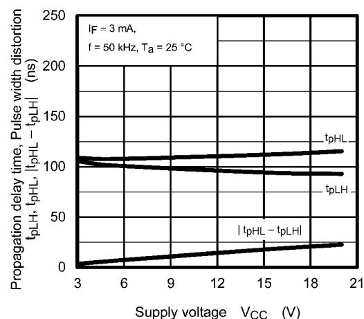
Fig. 12.2.21 t_{pHL} , t_{pLH} , |t_{pHL} - t_{pLH}| - V_{CC} (Test Circuit Fig. 12.1.8)
