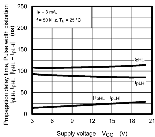
Fig. 12.2.15 t_{pHL} , t_{pLH} , |t_{pHL} - t_{pLH}| - V_{CC} (Test Circuit Fig. 12.1.7)
