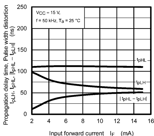
Fig. 12.2.17 t_{pHL} , t_{pLH} , |t_{pHL} - t_{pLH}| - I_F (Test Circuit Fig. 12.1.7)
