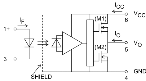
Fig. 5.1 Internal Circuit
