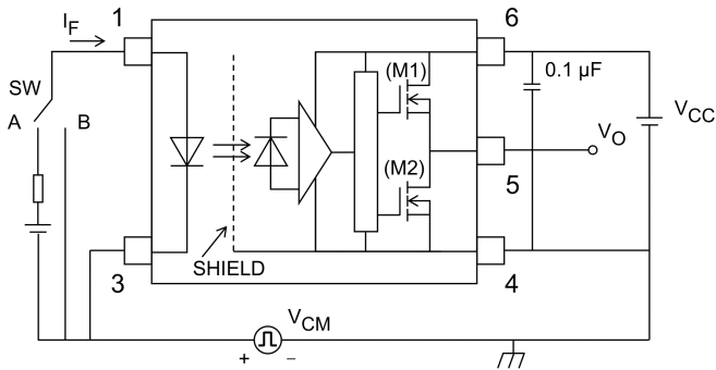
Fig. 12.1.8 Common-Mode Transient Immunity Test Circuit and Waveform
