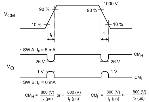
Fig. 12.1.8 Common-Mode Transient Immunity Test Circuit and Waveform
