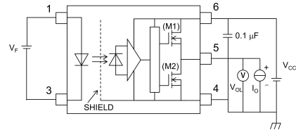
Fig. 12.1.4 V_{OL} Test Circuit
