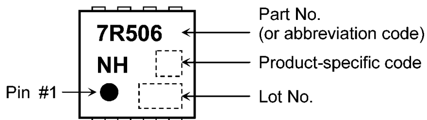
Fig. 7.1 Marking
