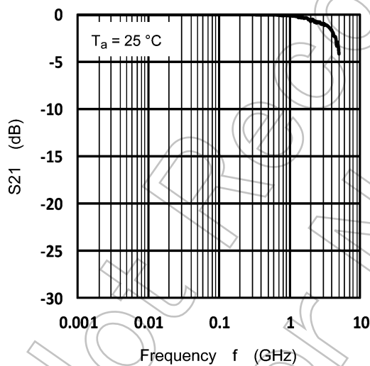
図 10.1 S_{21} - f
