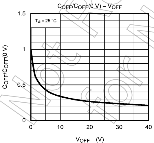
図 12.1.11 C_{OFF}/C_{OFF}(0\text{ V}) - V_{OFF}
