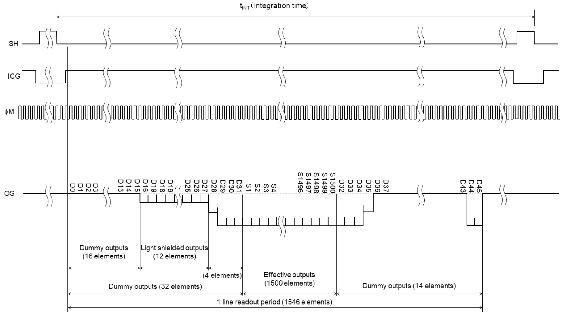
Timing Chart 1
