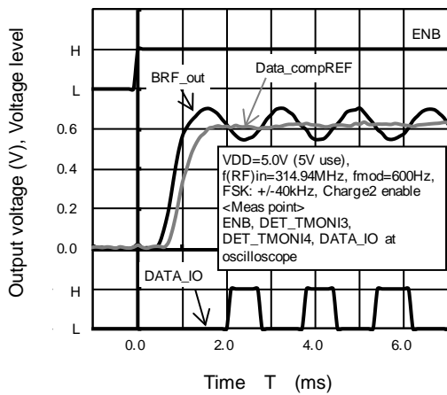
Data comparator, Response Characteristics of Rise Time FSK (bit rate = 600Hz)
