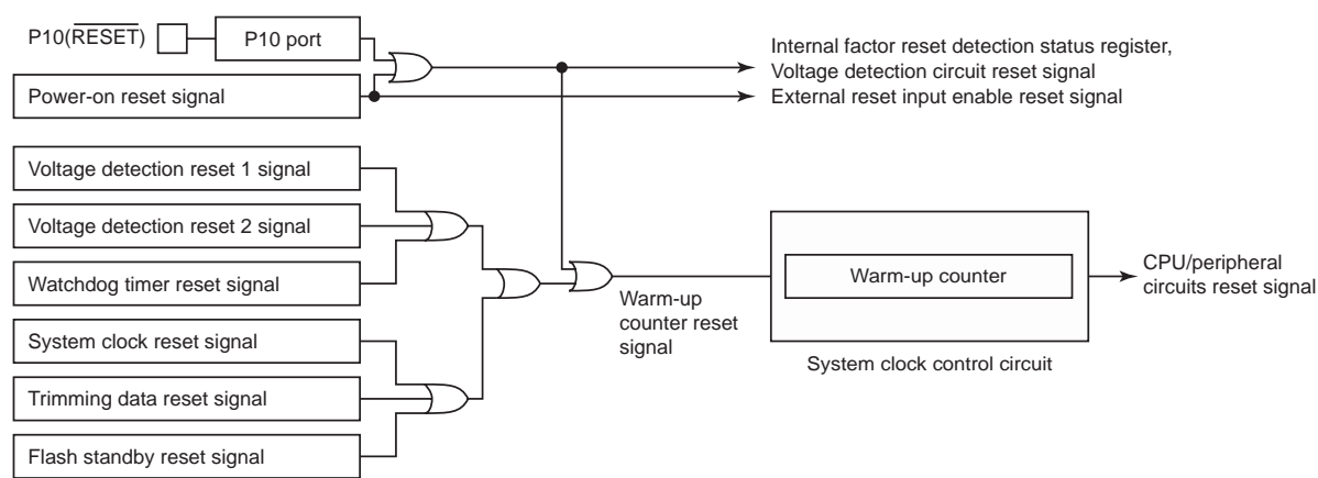
Figure 2-16 Reset Control Circuit
