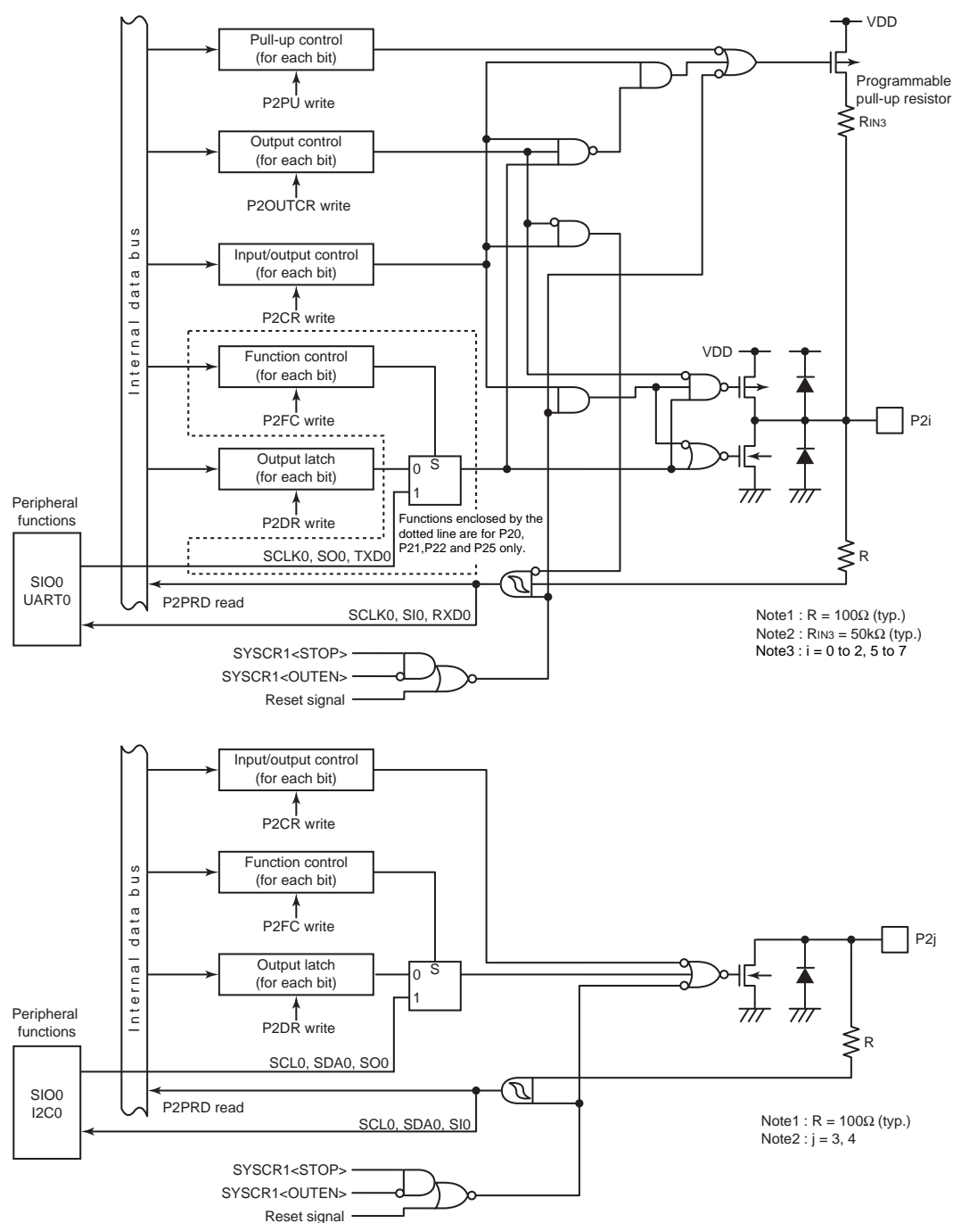
Figure 8-5 Port P2
