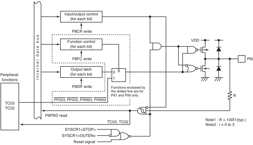
Figure 8-8 Port P8
