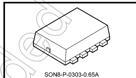
SON8-P-0303-0.65A
