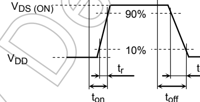
(c) V_{OUT}
