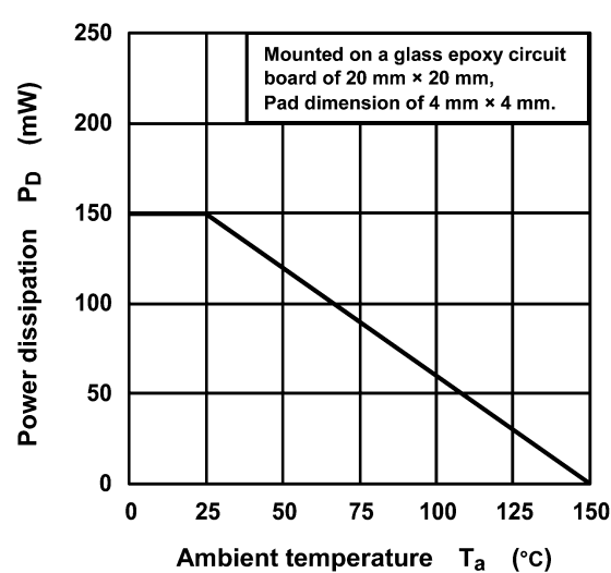
Fig. 7.4 P_D - T_a
