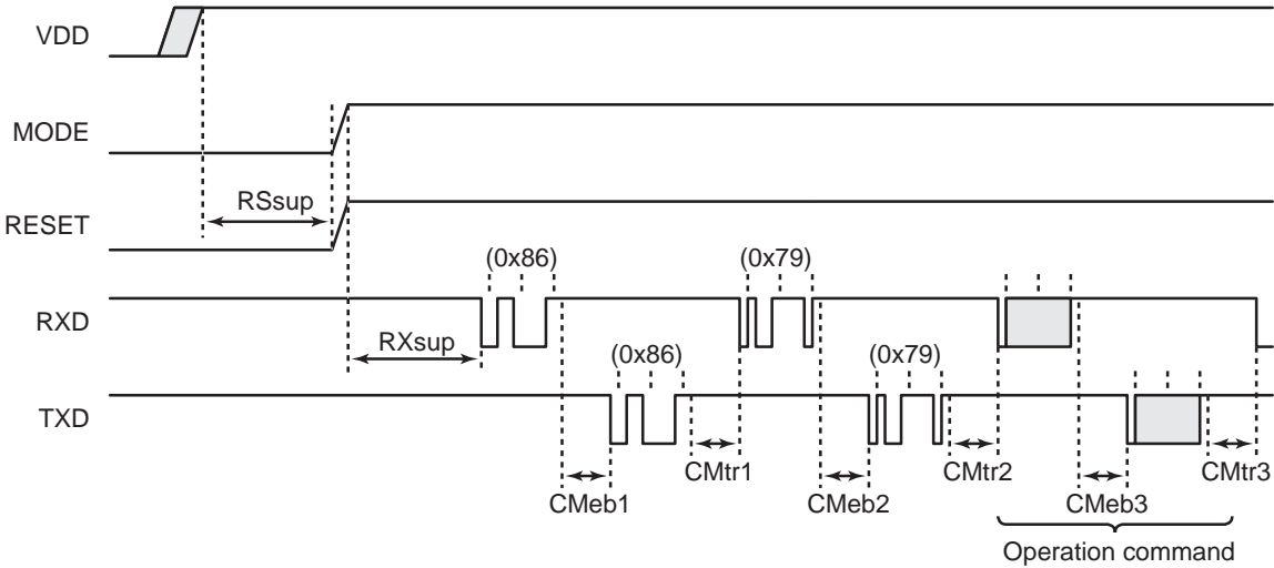
Figure 22-6 Reset Timing
