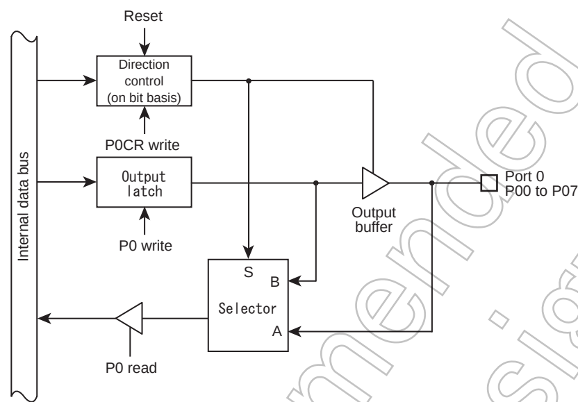
Figure 4-1 Port 0
