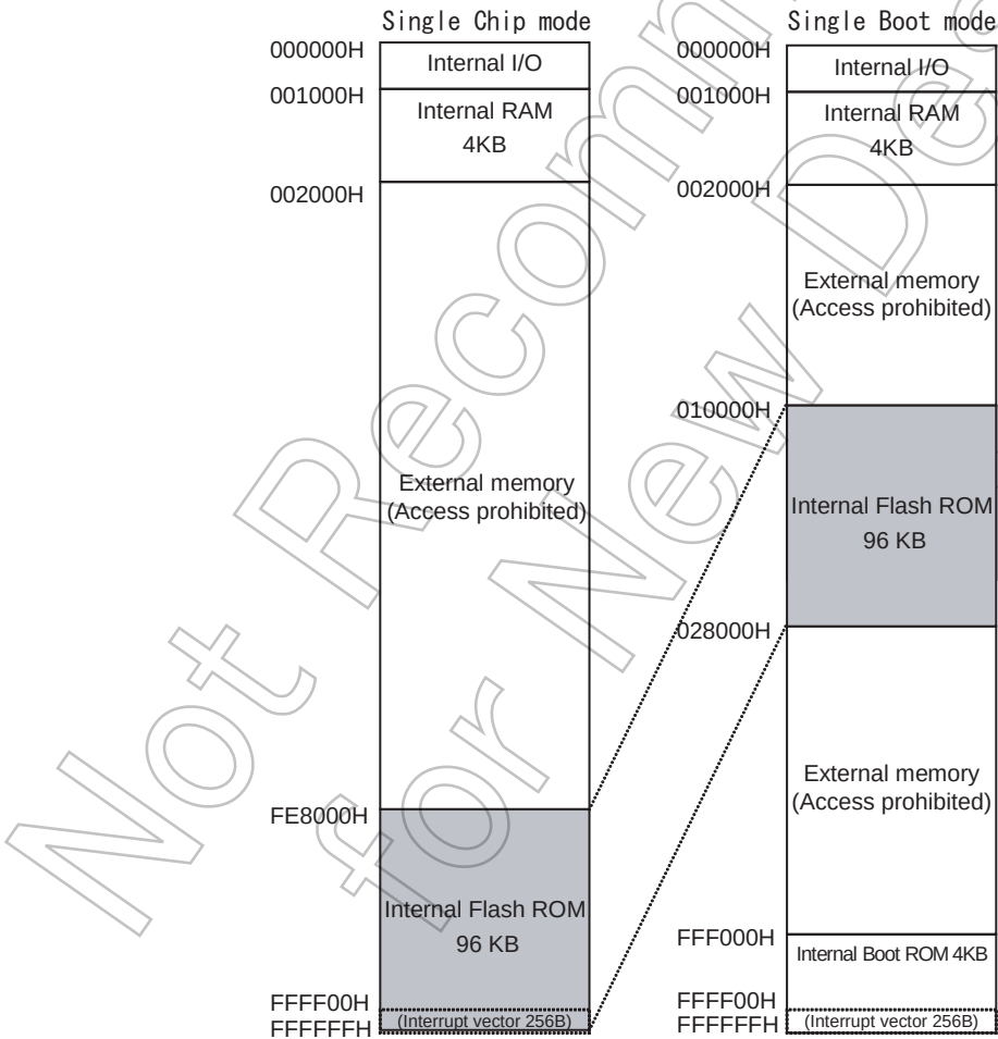
Figure 13-6 Comparison of Memory Maps
