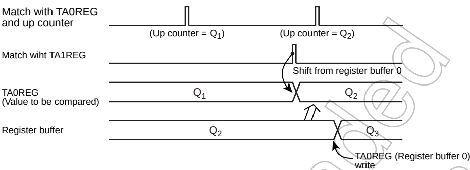
Figure 5-9 Operation of Register Buffer 0
