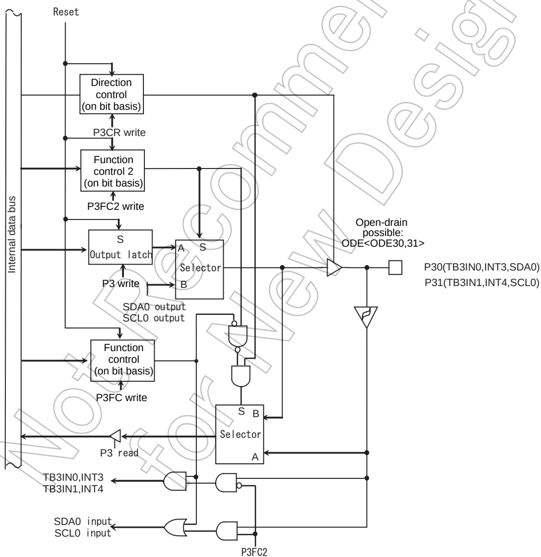
Figure 4-3 Port 30 and 31
