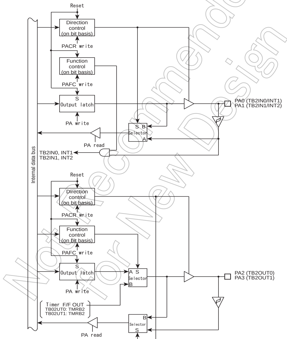
Figure 4-19 Port A
