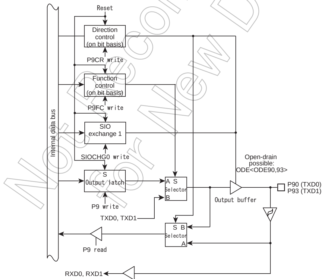
Figure 4-15 Port 90 and 93
