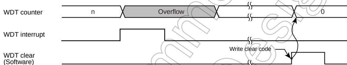
Figure 11-2 Normal Mode
