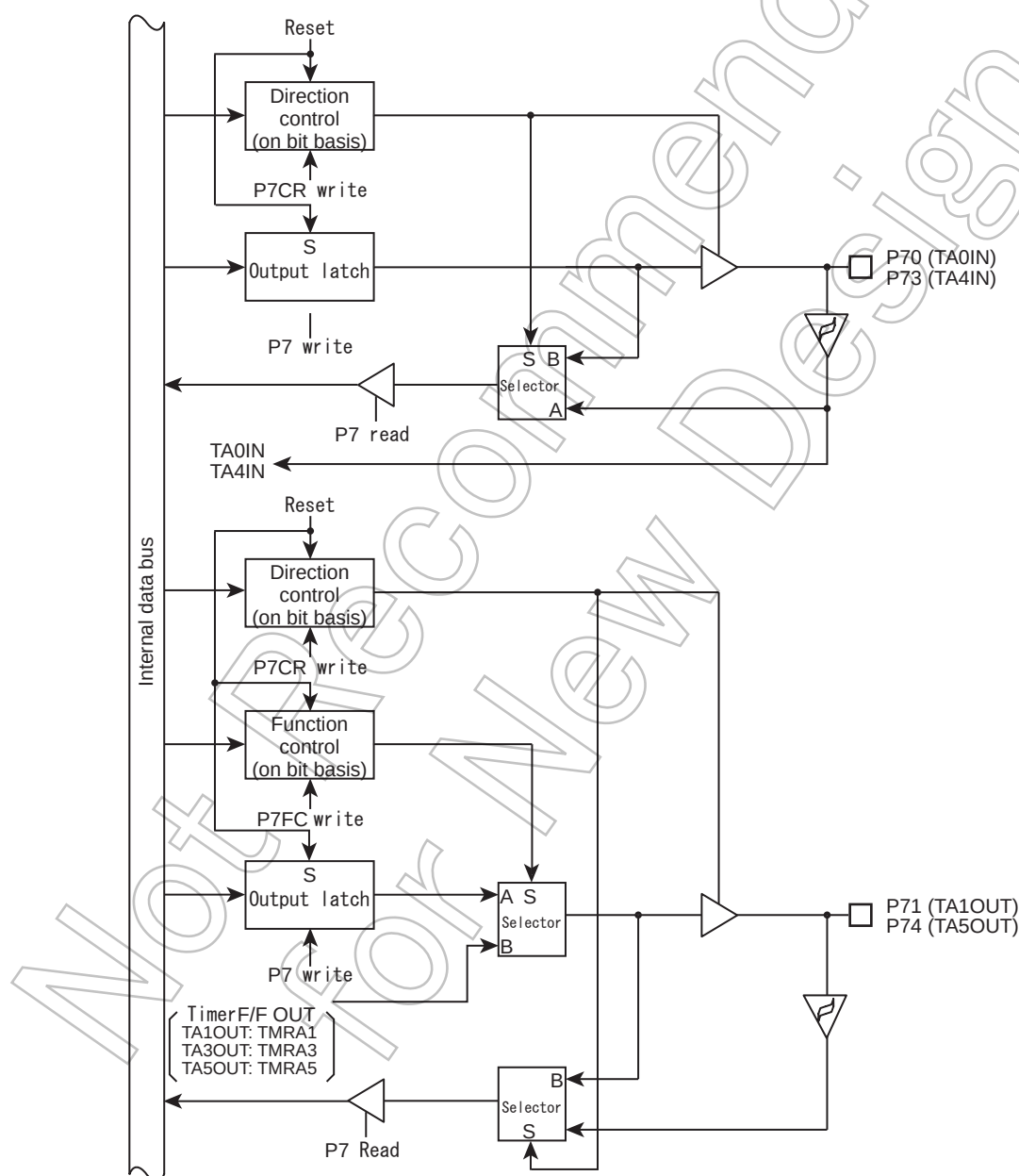
Figure 4-11 Port 70, 71, 73 and 74
