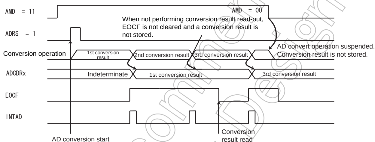
Figure 9-3 Repeat Mode
