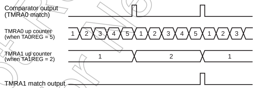
Figure 5-5 TMRA1 Count Up on Signal from TMRA0
