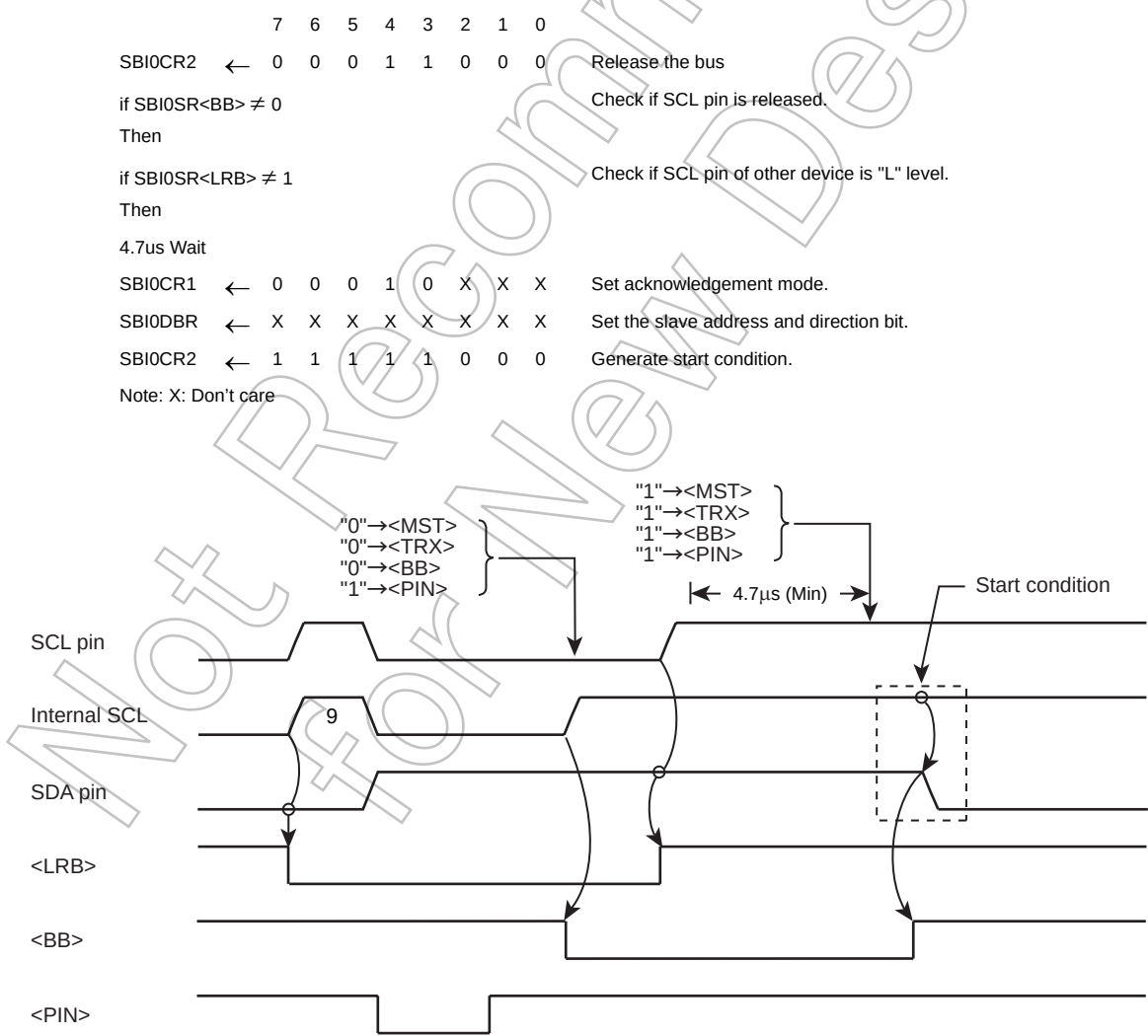
Figure 8-15 Timing Diagram for TMP91FU62 Restart
