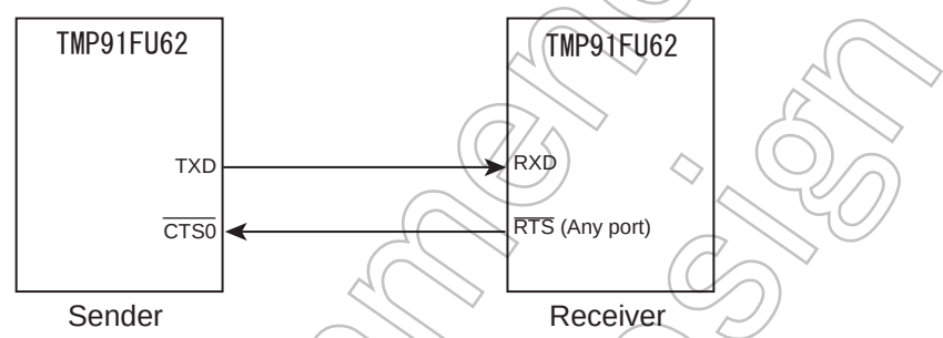
Figure 7-4 Handshake Function
