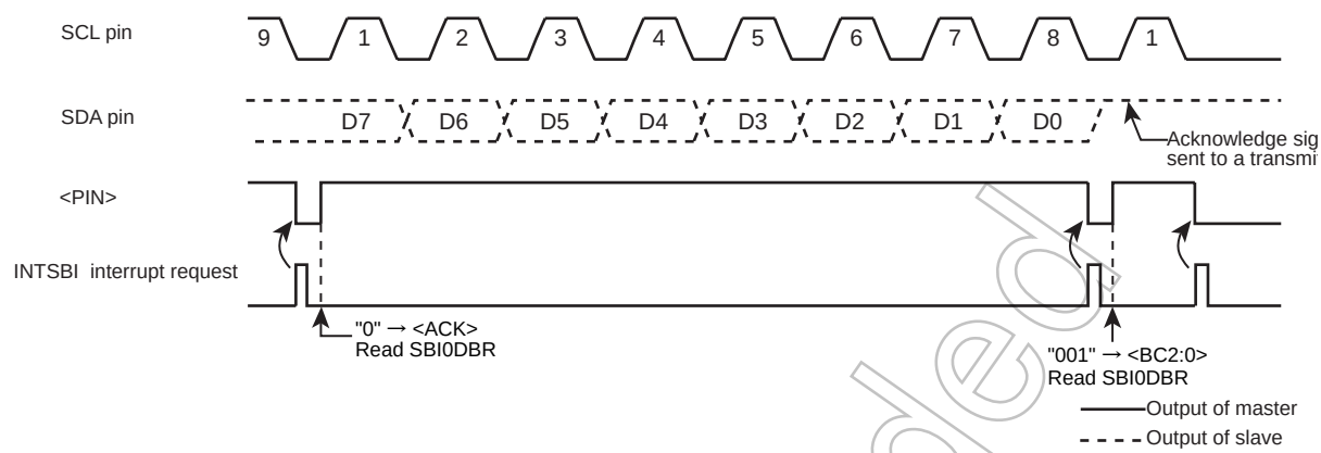
Figure 8-12 Termination of Data Transfer in Master Receiver Mode
