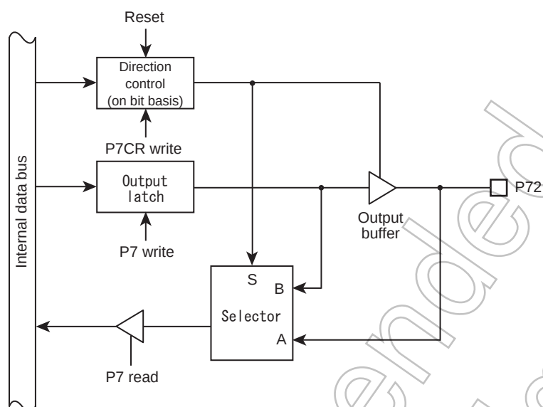
Figure 4-12 Port 72
