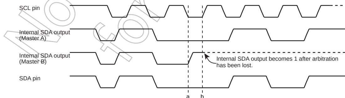
Figure 8-7 Arbitration Lost
