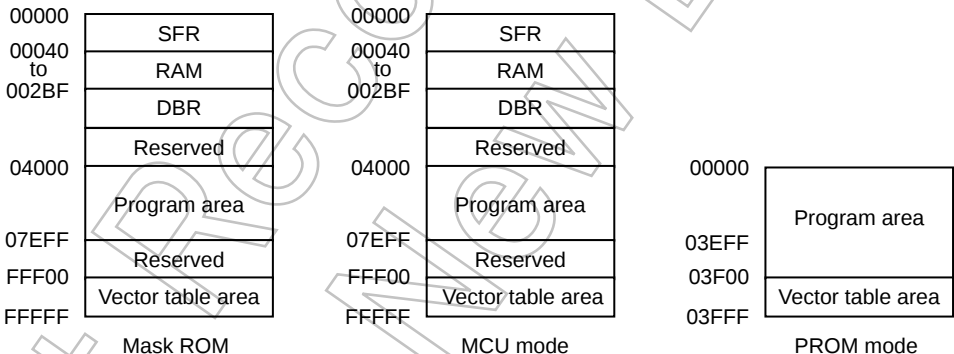
Figure 16-1 Program Memory Area
