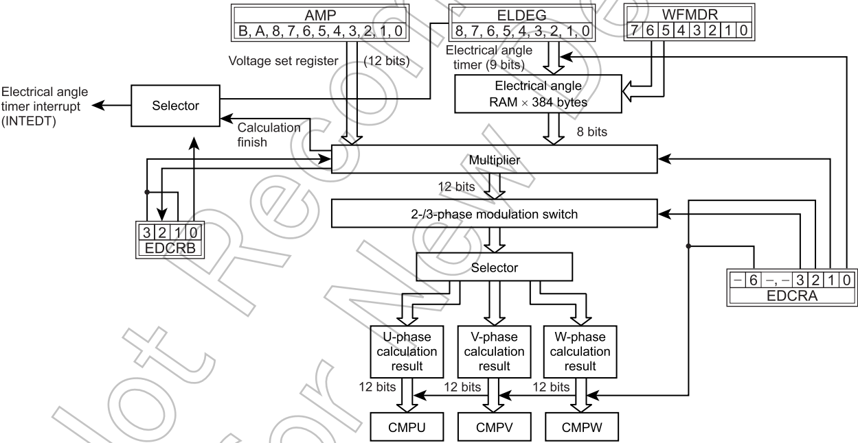
Figure 12-16 Waveform Arithmetic Circuit
