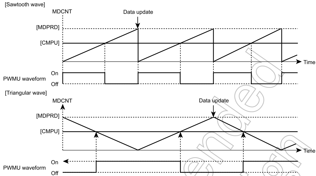
Figure 12-9 PWM Waveforms
