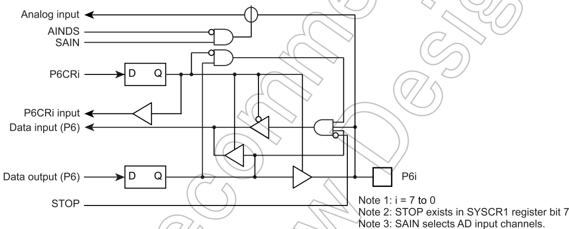
Figure 5-6 Port P6
