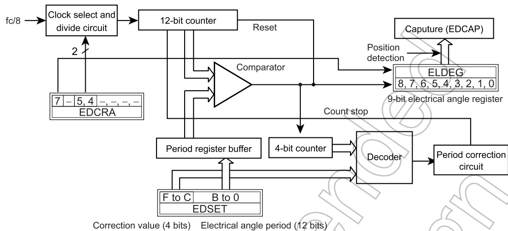
Figure 12-15 Electrical Angle Timer Circuit
