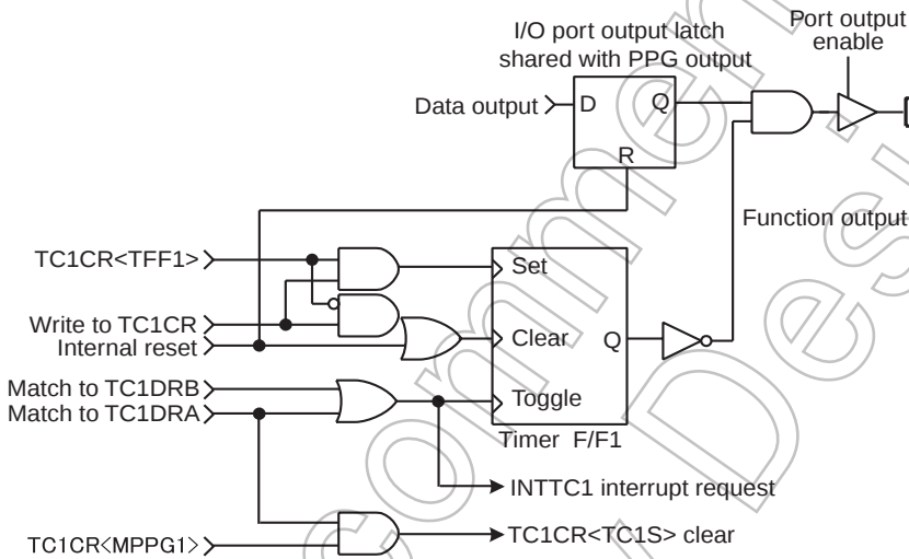
Figure 8-7 \overline{\text{PPG}} Output
