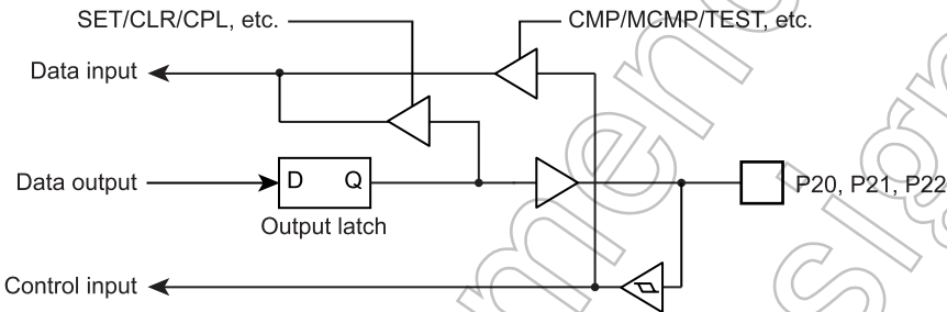
Figure 5-3 Port P2
