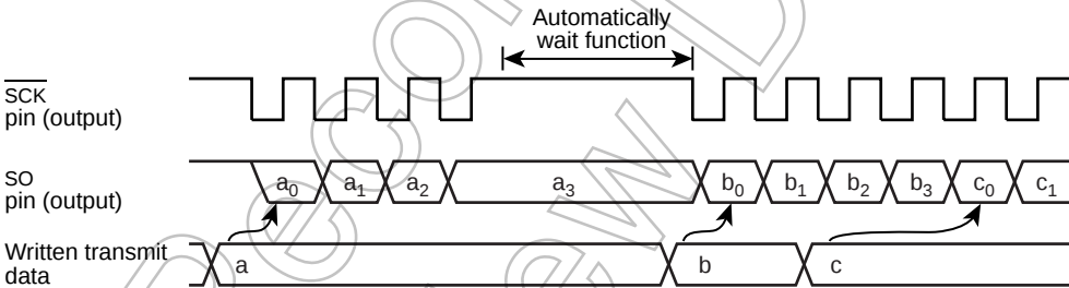
Figure 14-3 Automatic Wait Function (at 4-bit transmit mode)
