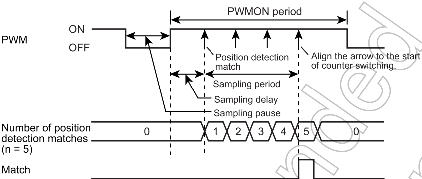
Figure 12-5 Position Detection Sampling Timing with the PWMON Period Selected
