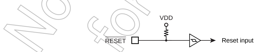
Figure 2-12 Reset Circuit
