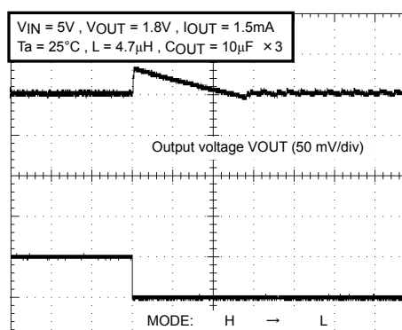
Mode Switching I_{OUT} = 1.5mA (synchronous→non-synchronous)
