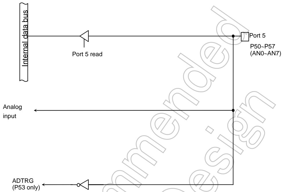
Figure 3.5.13 Port 5
