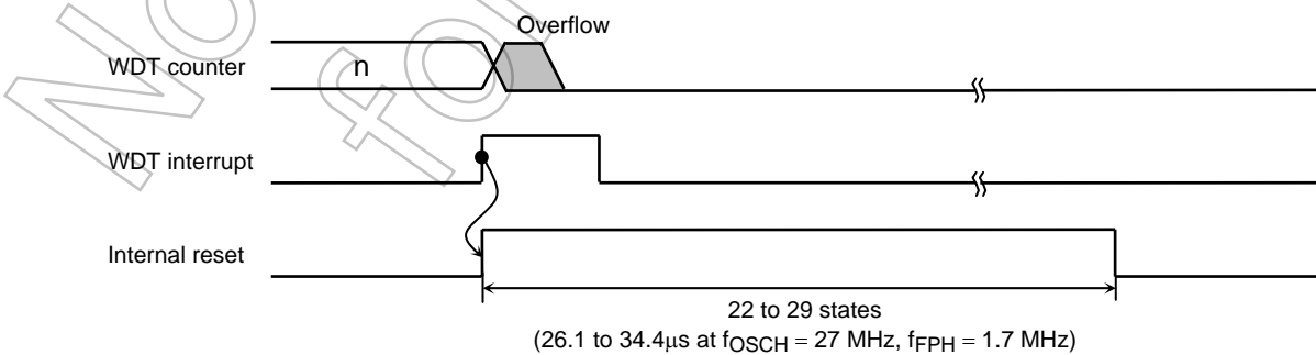
Figure 3.12.3 Reset Mode
