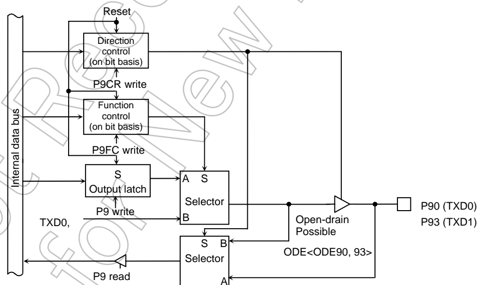
Figure 3.5.26 Ports 90 and 93
