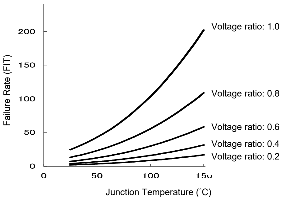
Figure 1.2.1 MIL-HDBK-217-Based Derating
