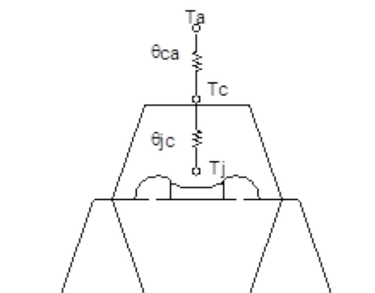
Figure 3.3.1 Thermal Resistance of Package
