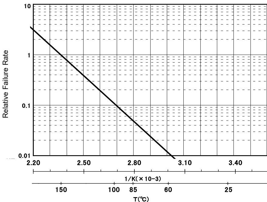
Figure 1.2.2 Transistor Derating Curve
